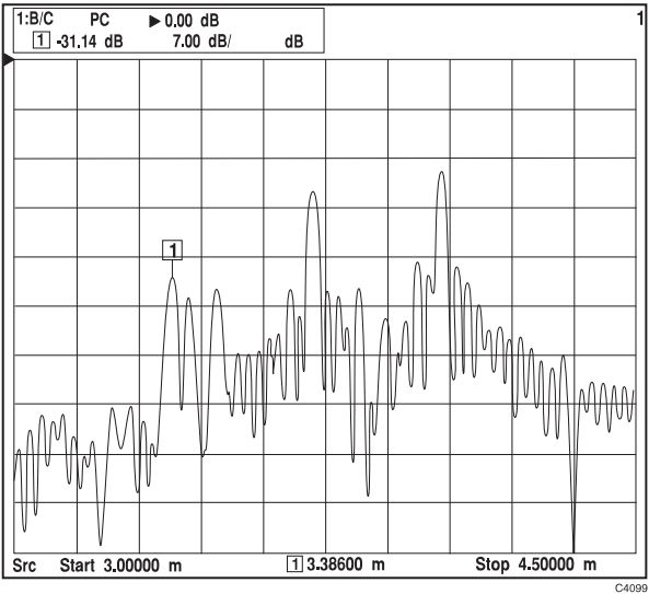
Fig. 2-41 Display of sub-range
