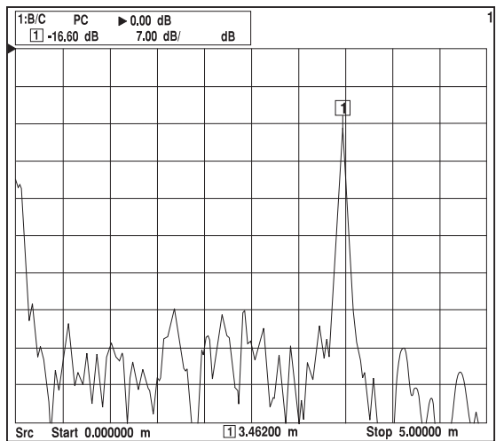
Fig. 2-40 Effect of windowing
