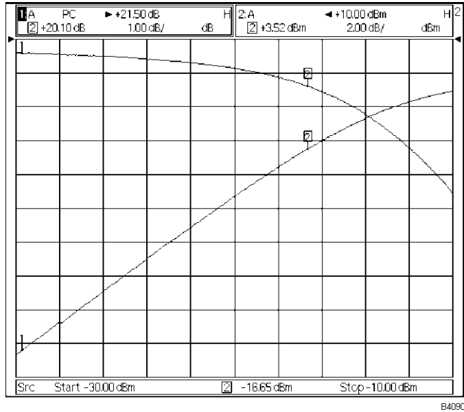
Fig. 2-13 Gain compression measurement
