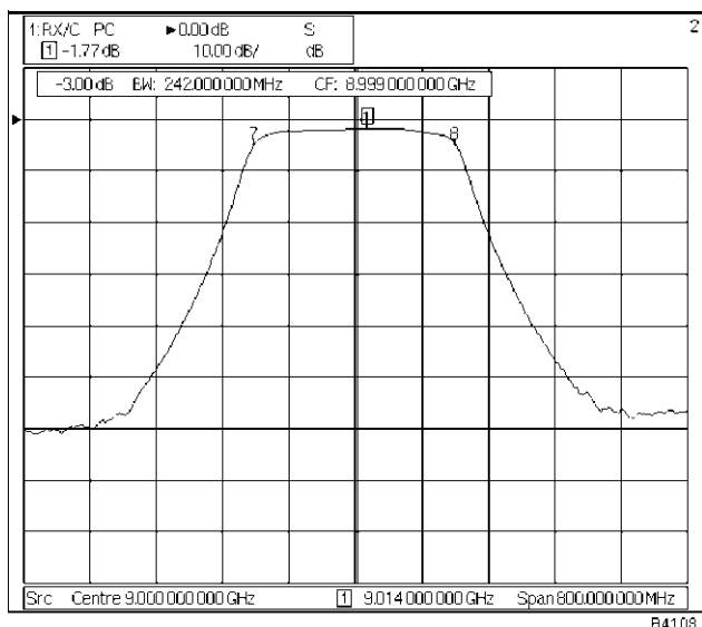
Fig. 2-17 High dynamic range, ratioed insertion loss measurement
