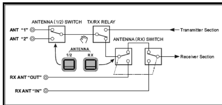
Simplified diagram of FT2000 Aerial Selection
