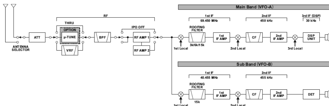
FT2000 RX Block Diagram showing common front end.
