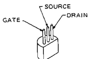
2SK19TM-GR
