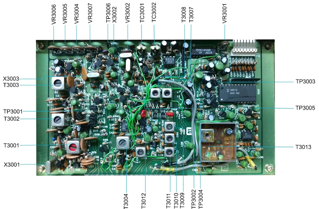
LOCAL UNIT (PB-2253 B)
