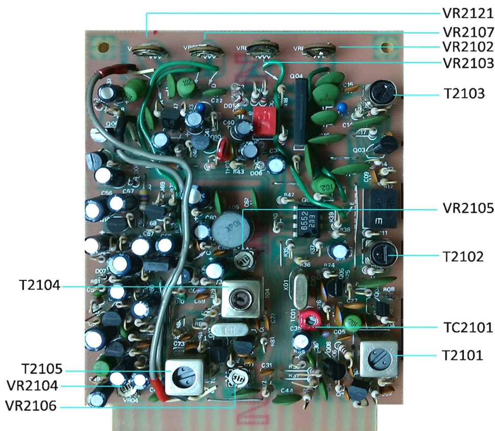
FM UNIT (PB-2254)
