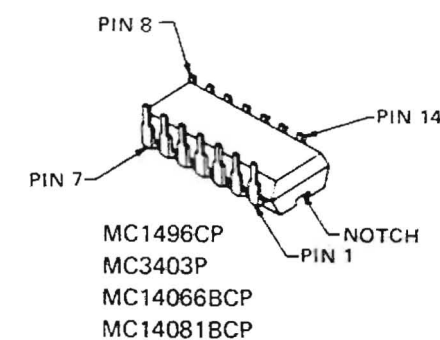
Viewed from component side
