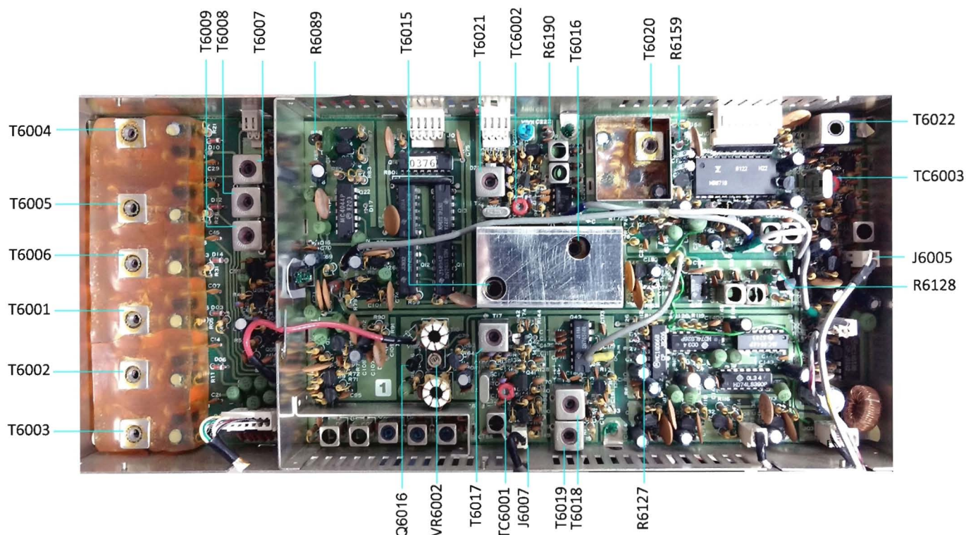
PLL UNIT (PB-2257, early model)
