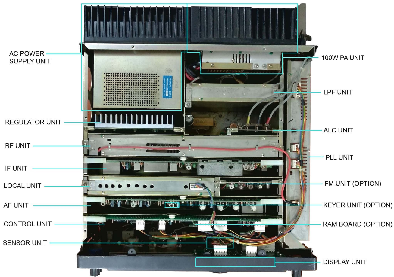
TOP VIEW
