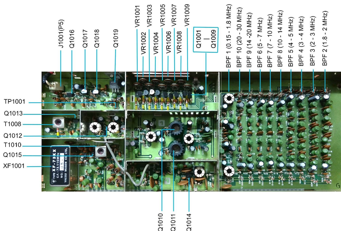
RF UNIT (PB-2256)
