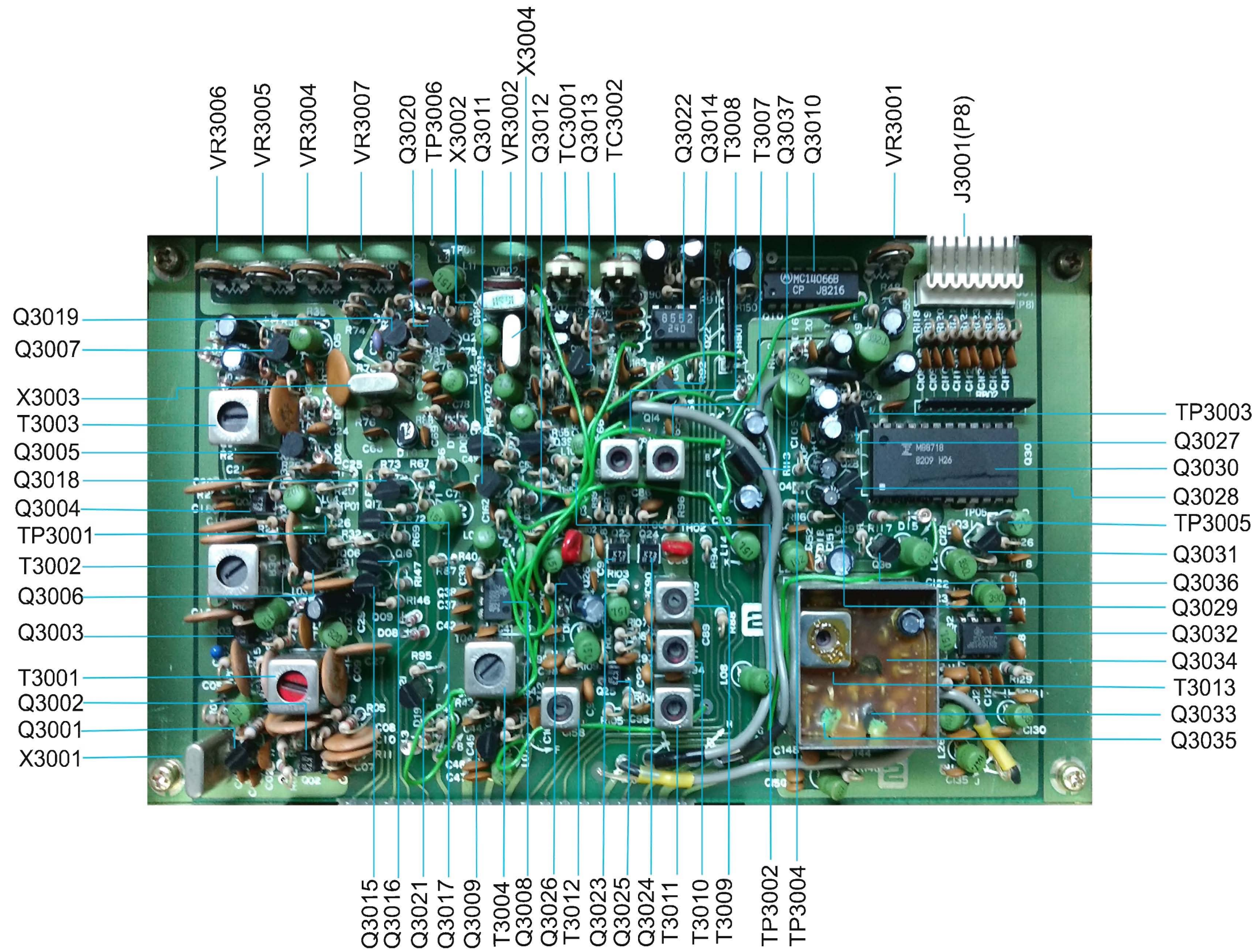
LOCAL UNIT (PB-2253 B)
