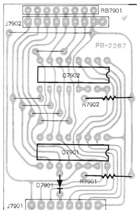
Viewed from foil side
