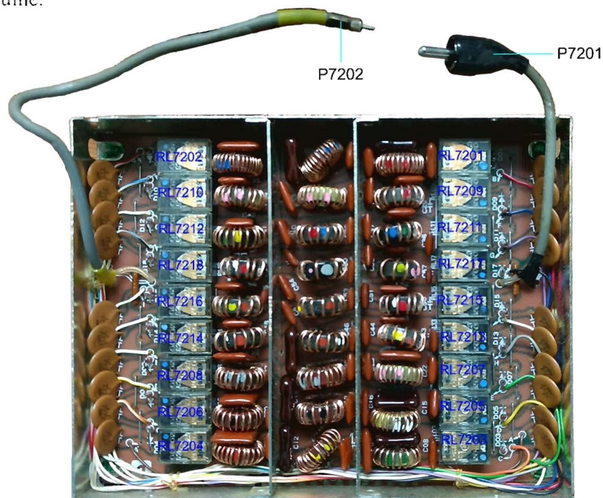
LPF UNIT (PB-2259)
