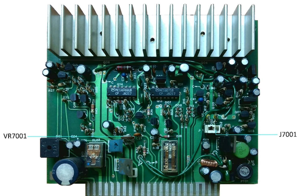
REG UNIT (PB-2258)
