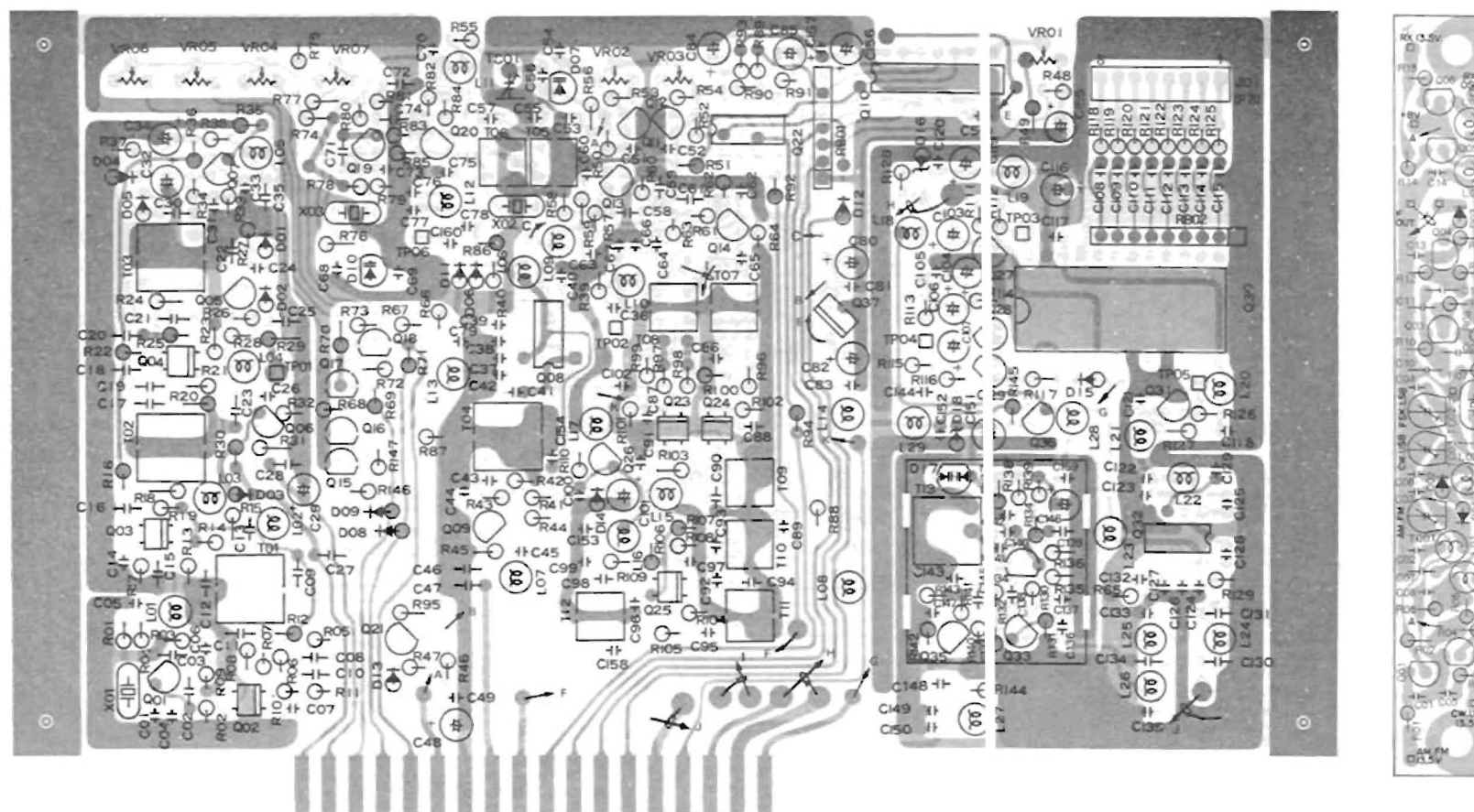
Viewed from component side
