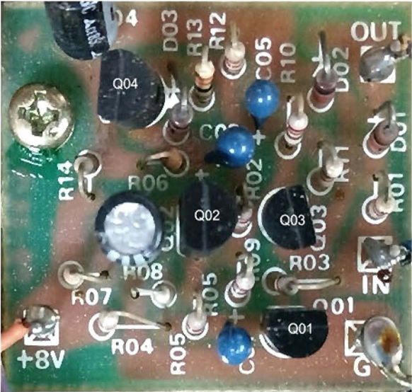
Components side view
