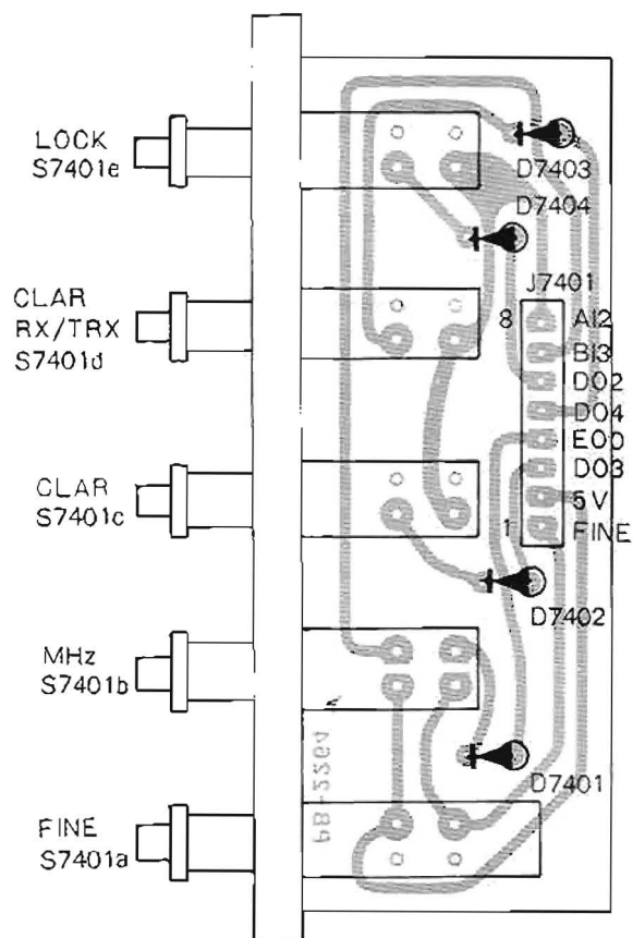
Viewed from component side
