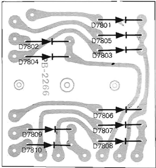
Viewed from foil side
