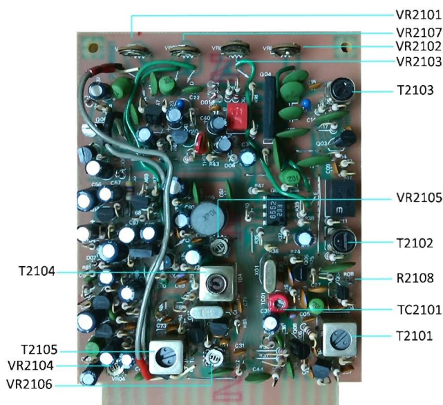
FM UNIT (PB-2254)
