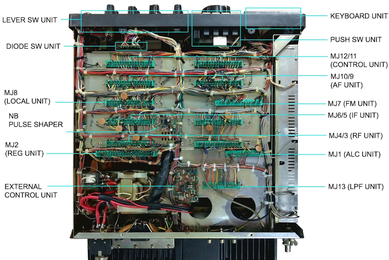
BOTTOM VIEW
