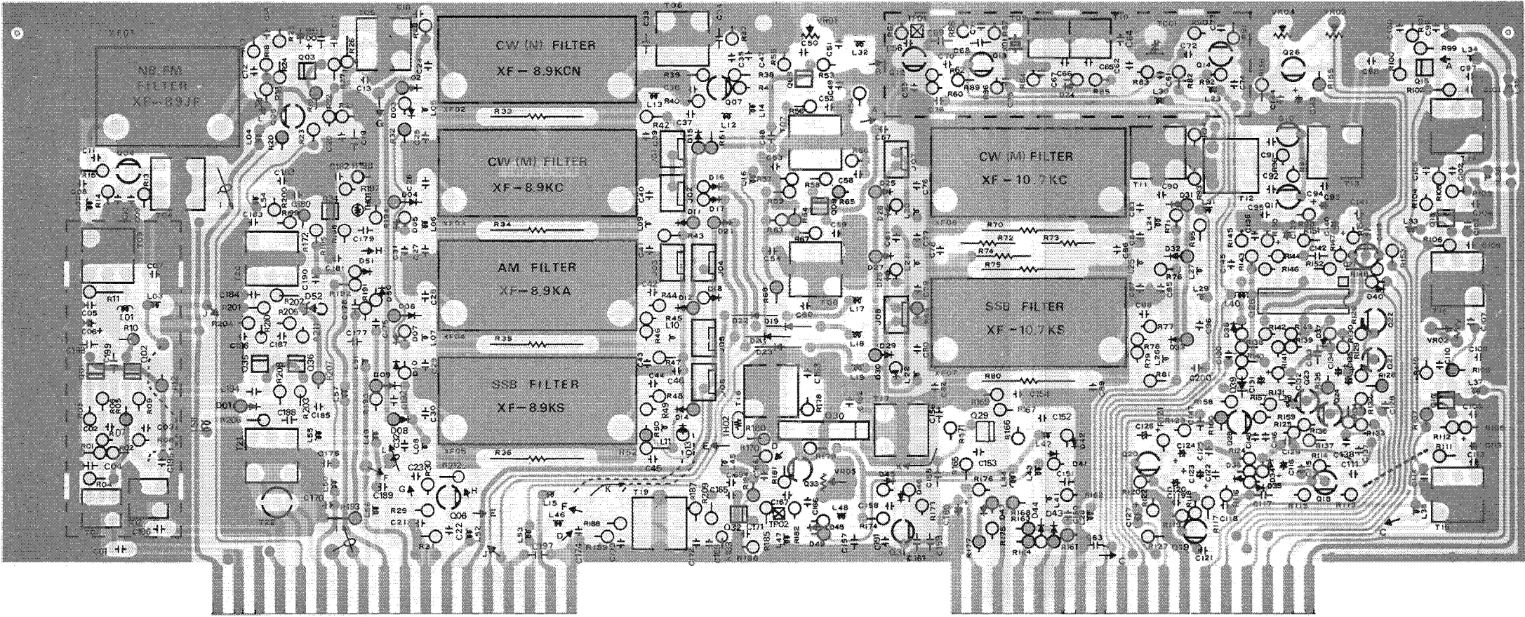
Viewed from component side
