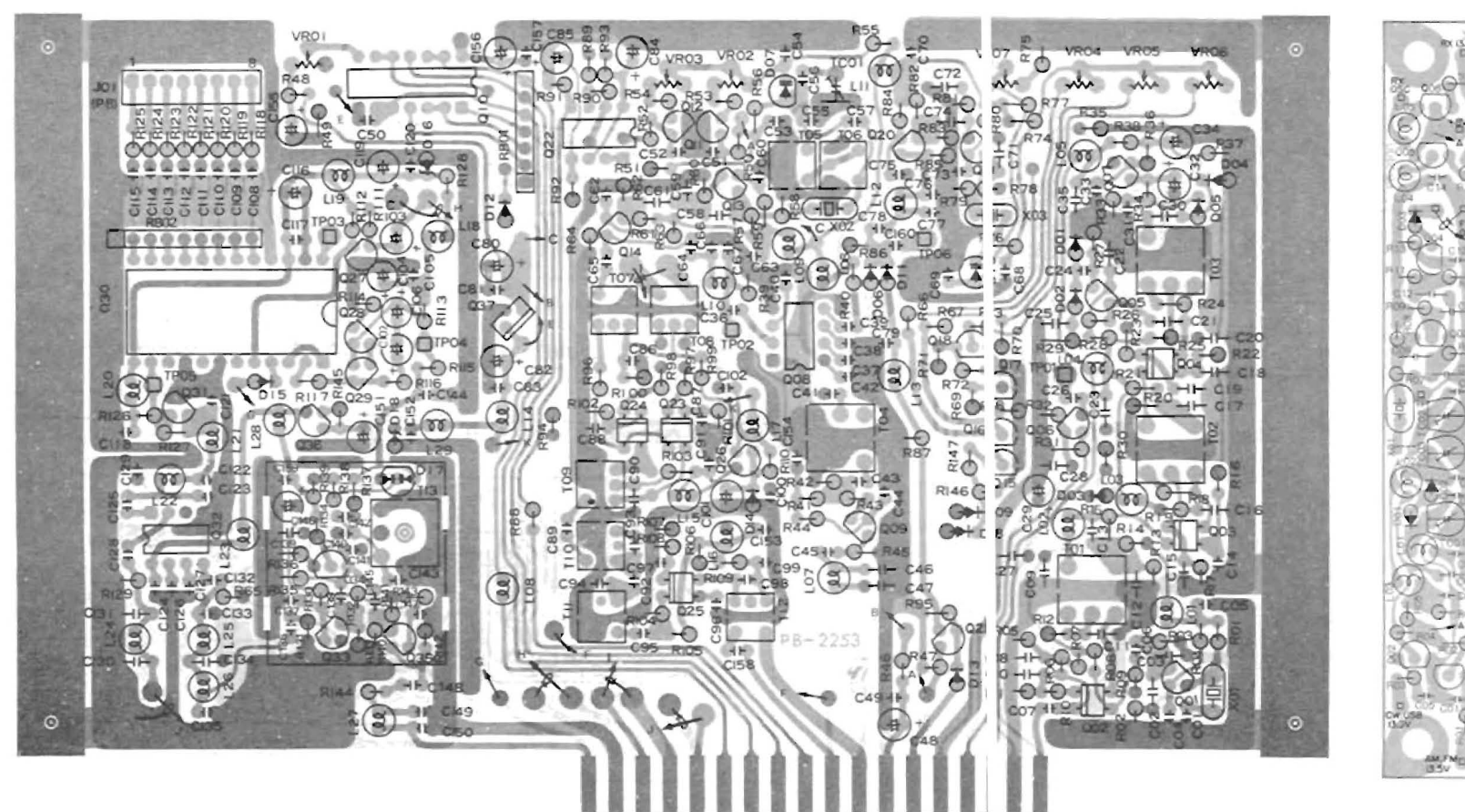
Viewed from solder side
