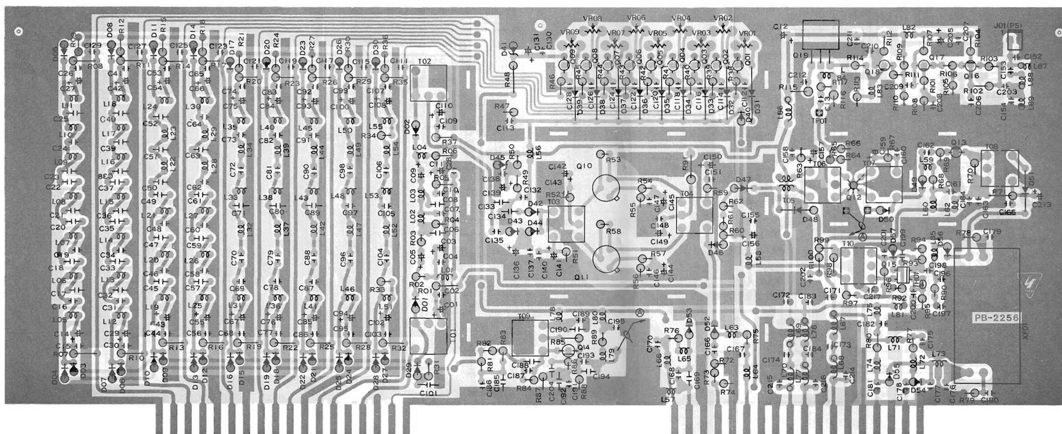
Viewed from solder side
