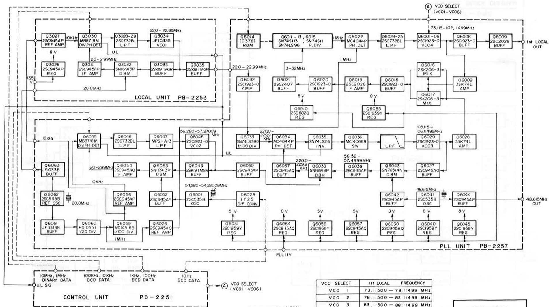
FT - ONE PLL BLOCK DIAGRAM
