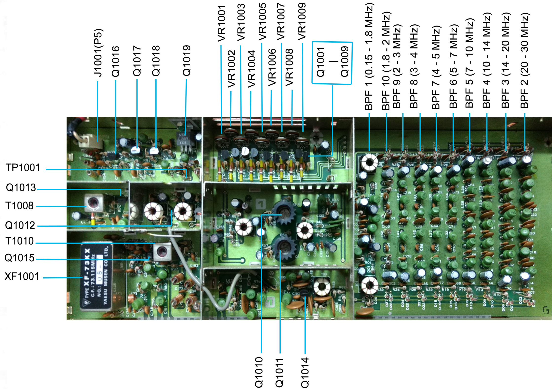
RF UNIT (PB-2256)
