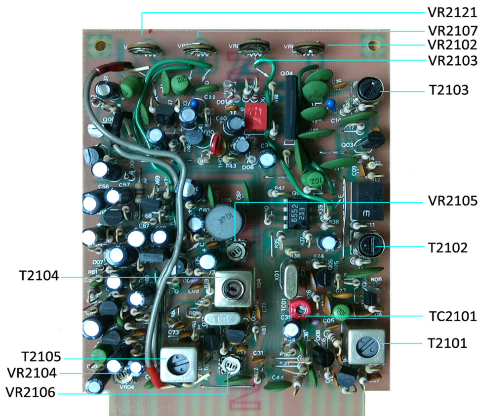
FM UNIT (PB-2254)
