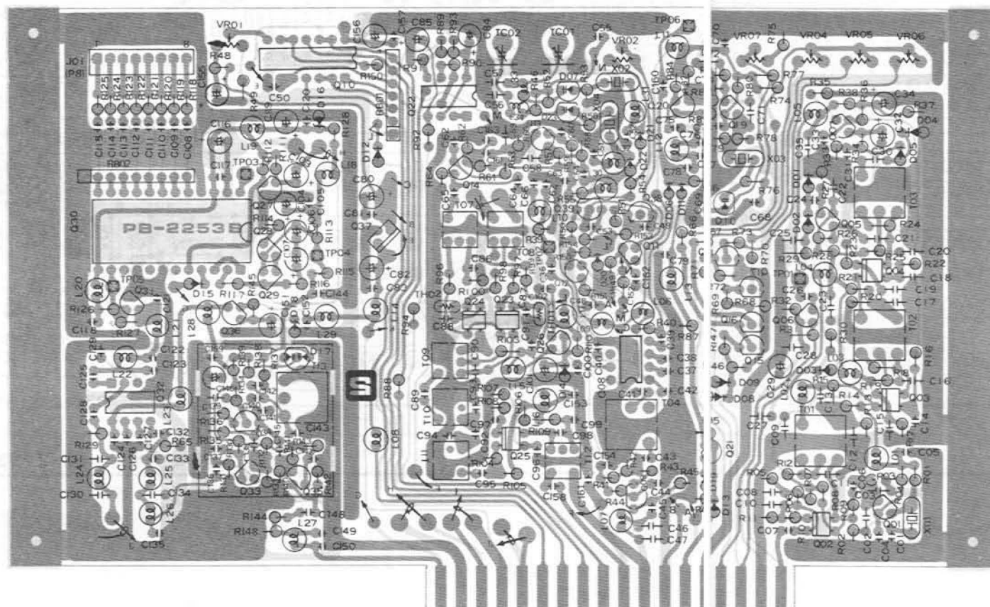
Viewed from solder side
