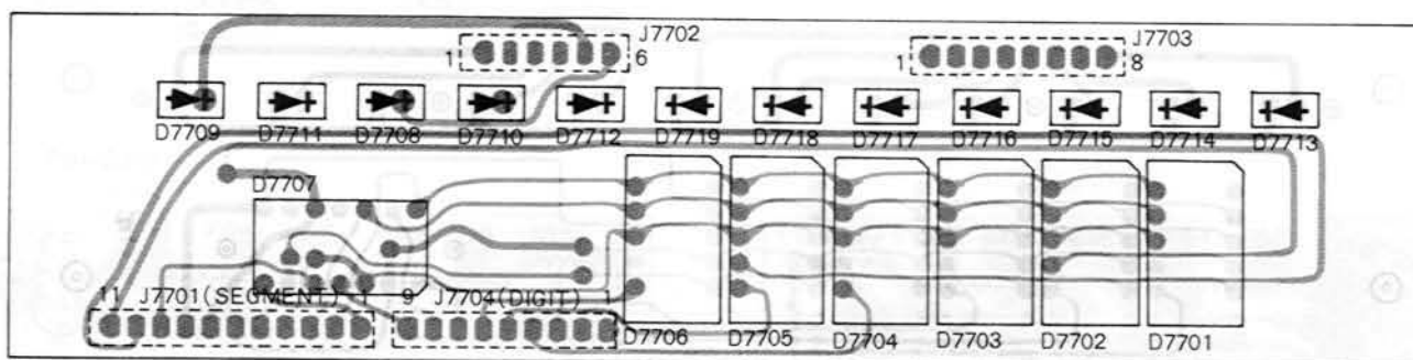
Viewed from solder side
