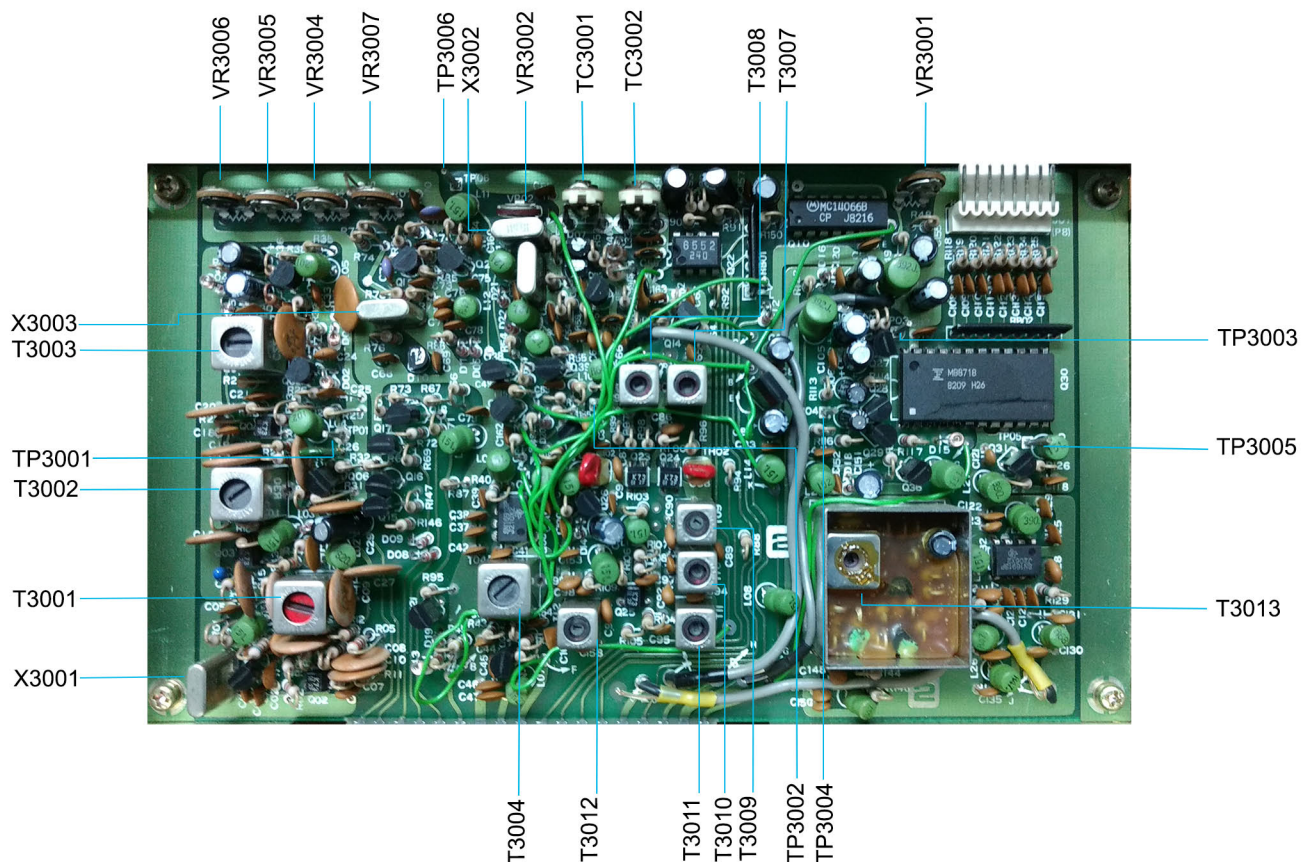
LOCAL UNIT (PB-2253 B)
