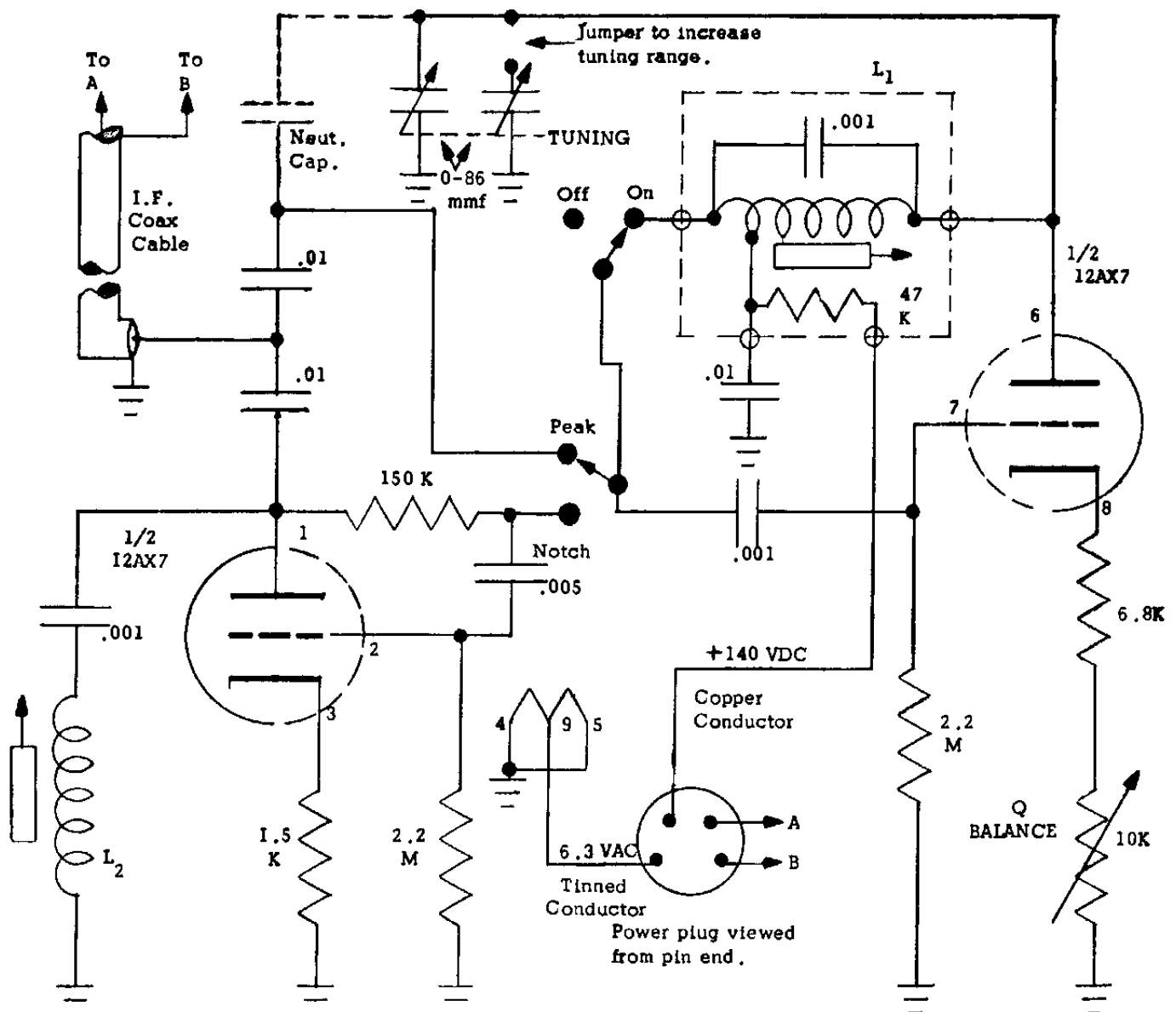
SCHEMATIC DIAGRAM OF 2-AQ
