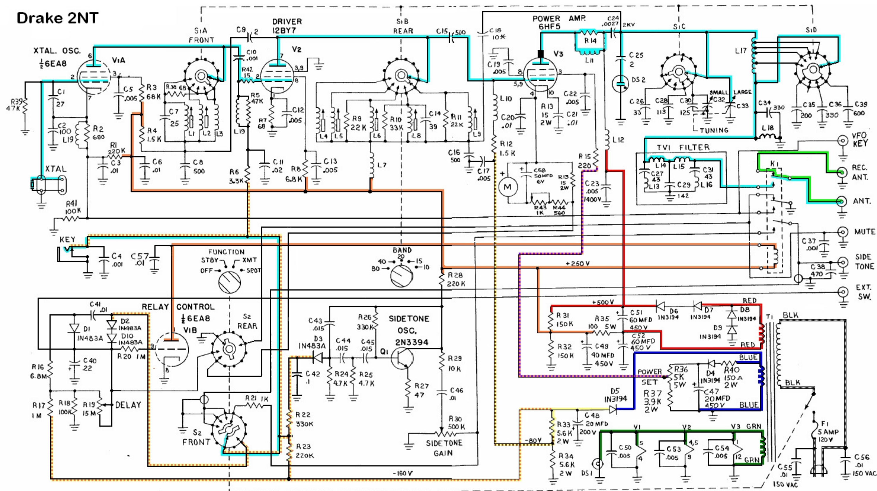
SCHEMATIC DIAGRAM MODEL 2-NT TRANSMITTER
