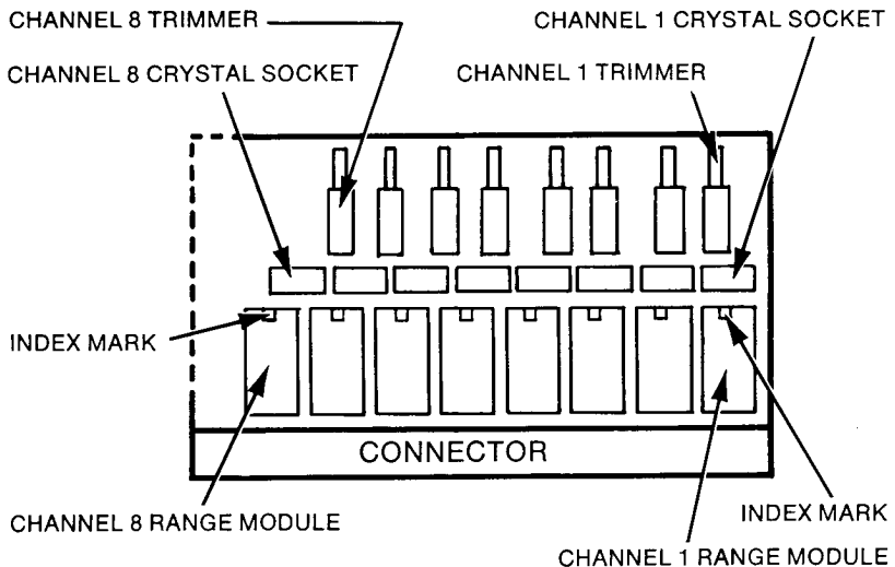
Figure 2—AUX7 Module
