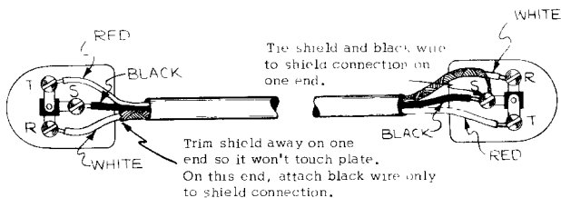
FIG 2 C-4 to Transmitter Cable Assembly
