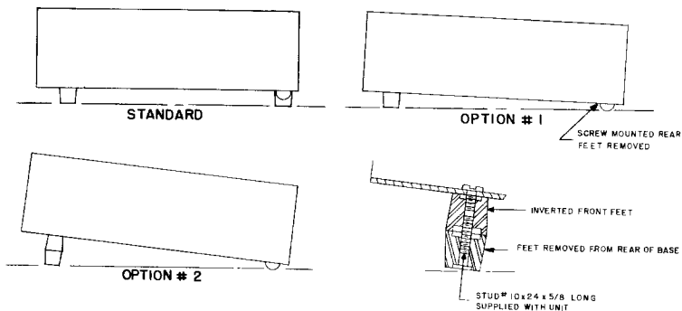
FIG. 3 Viewing Angle Options
