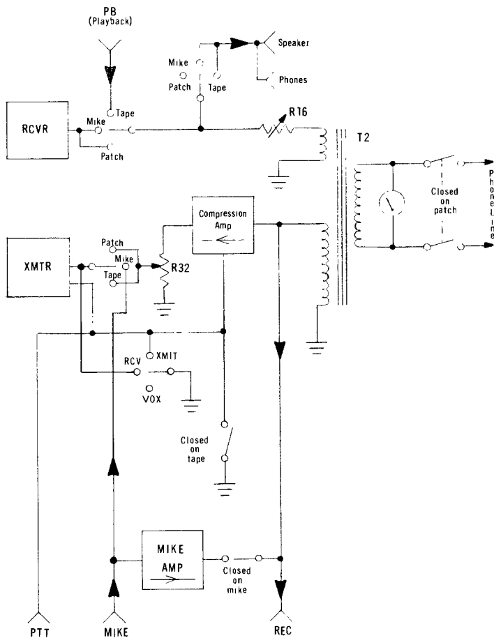
FIG.7 Block Diagram of PHONE PATCH
