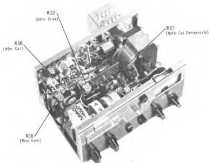
FIG. 10 Top View
