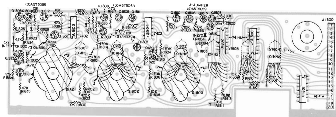
Figure 5-27. Counter No. 1, P/N 689-1800 (A18)
