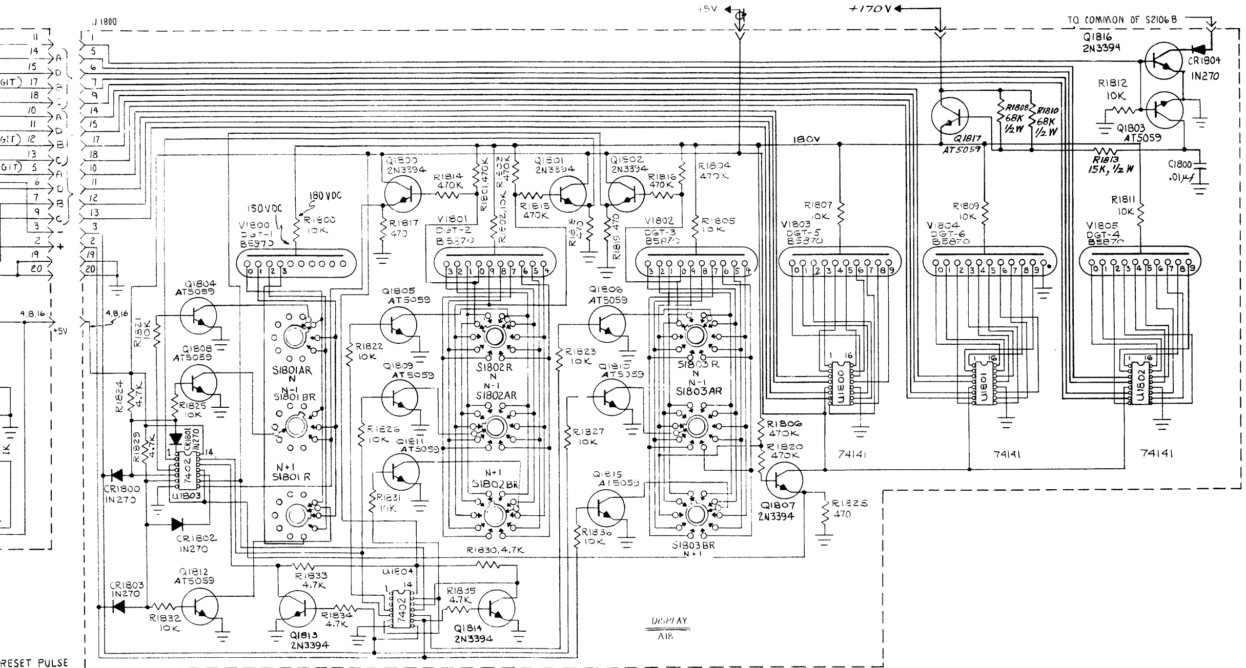
Figure 5-35. Counter Schematic
