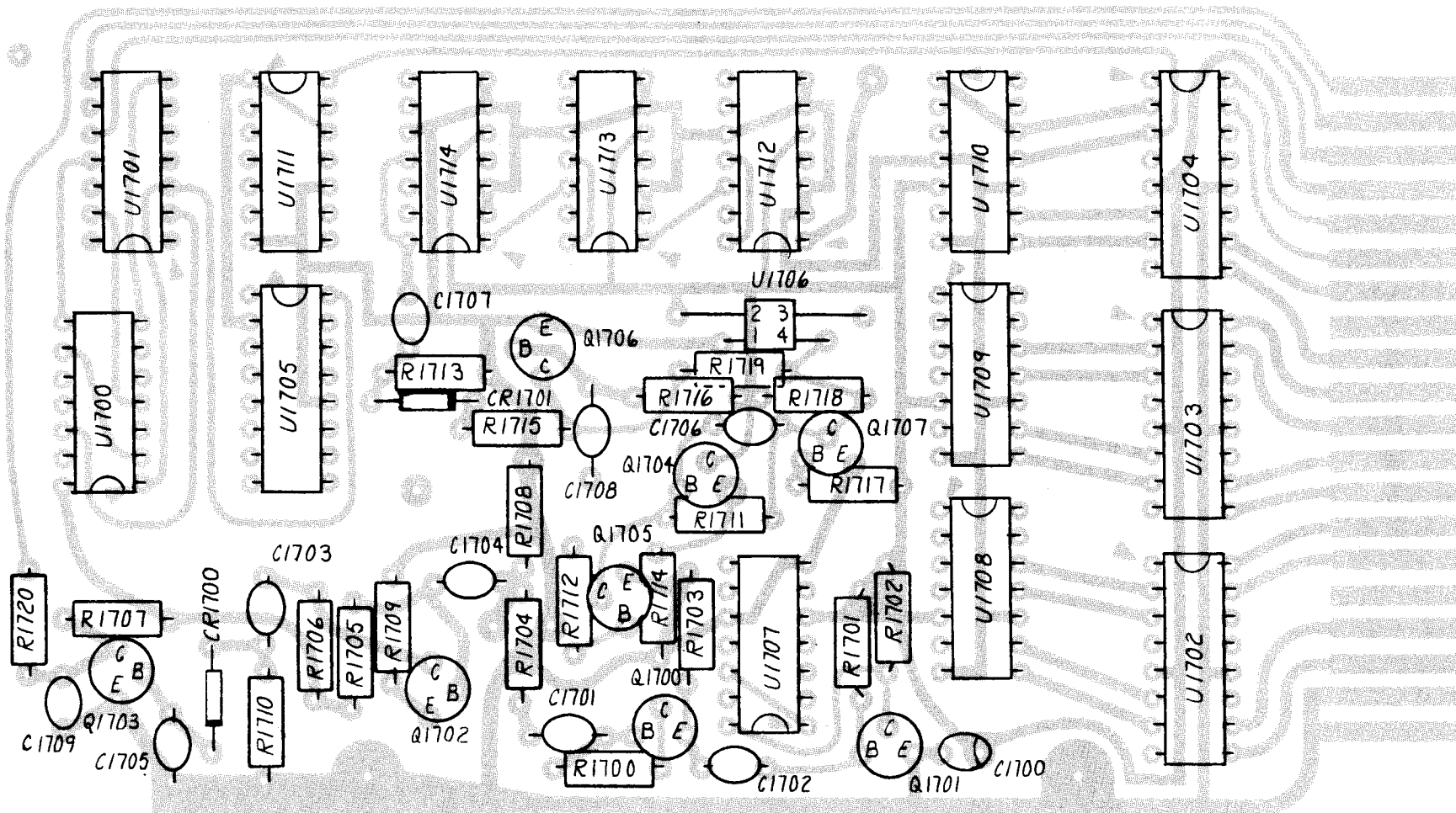
Figure 5-25. Counter (A17)
