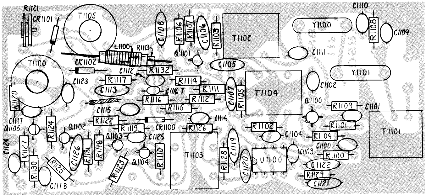
Figure 5-19. First IF and Noise Blanker, P/N 689-1100 (A11)
