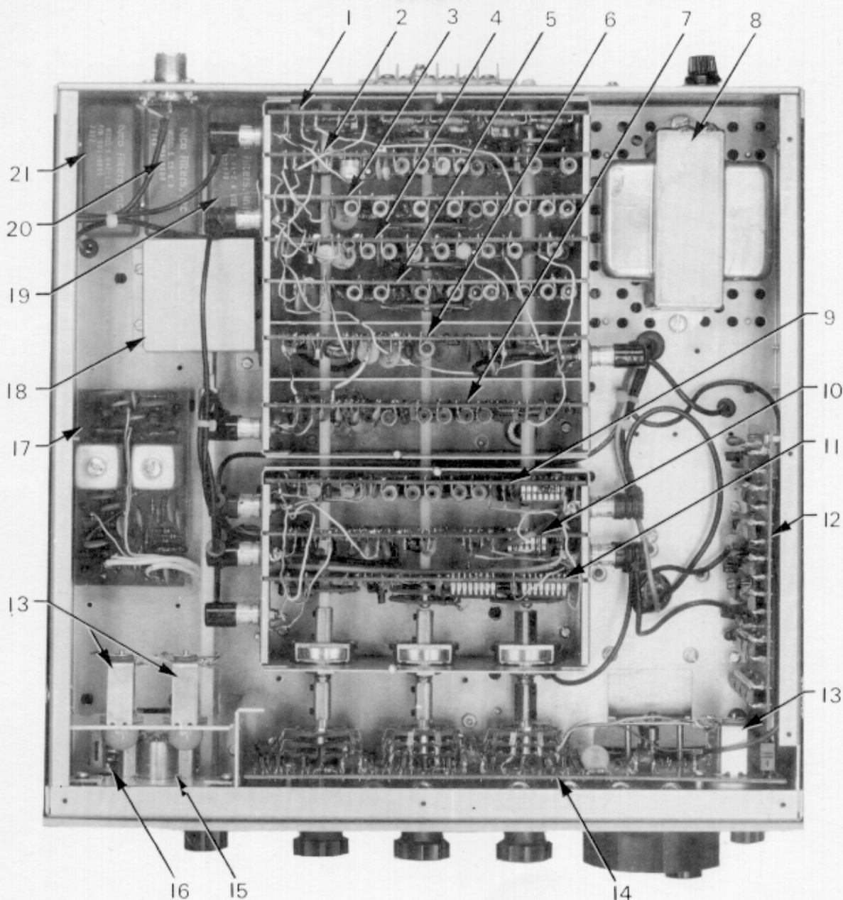
Figure 5-7. Component Locations, Top View
