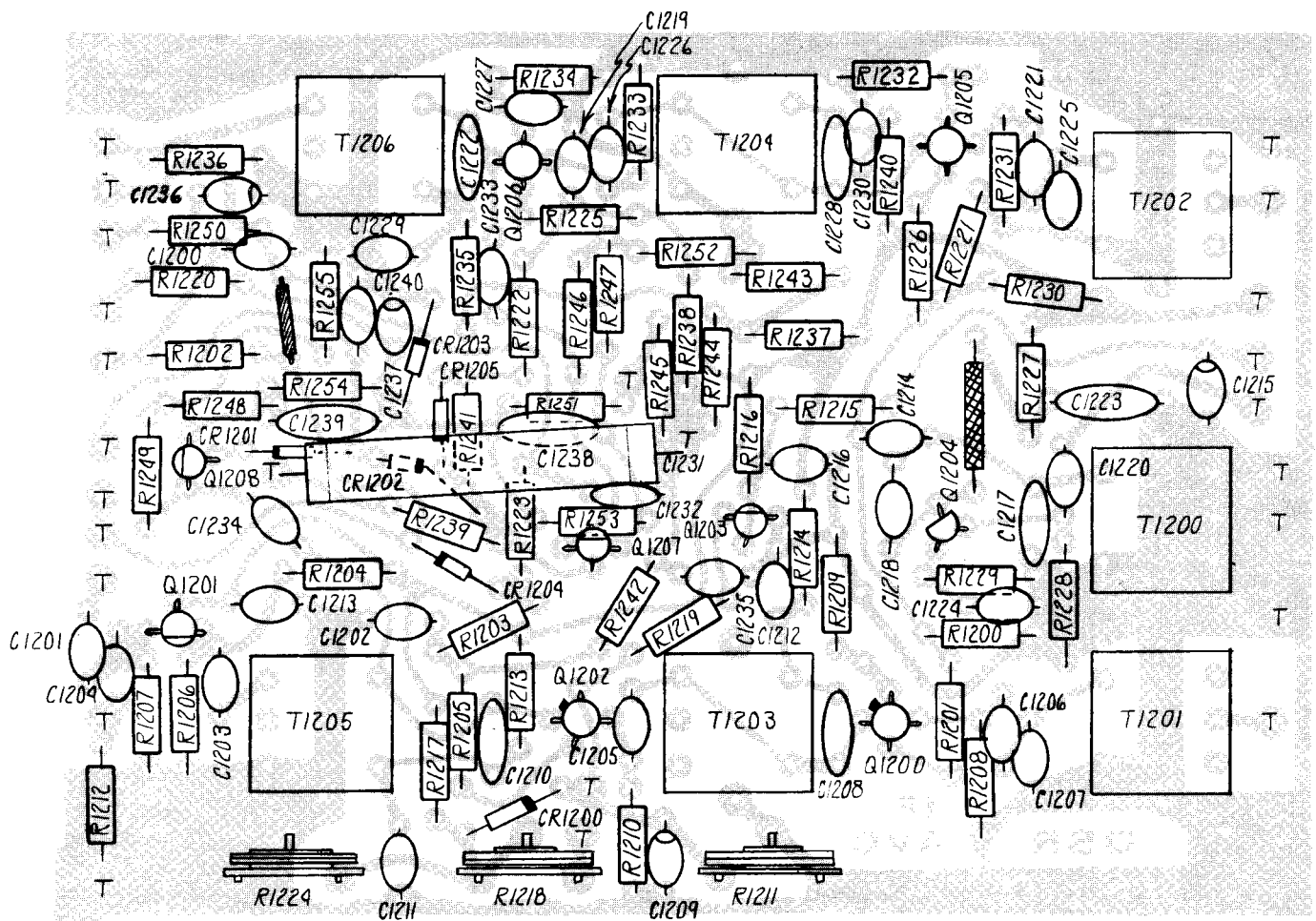
Figure 5-20. Second IF and AVC, P/N 689-1200 (A12)
