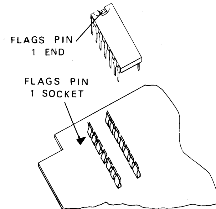
Figure 5-2. Proper Installation of Integrated Circuits
