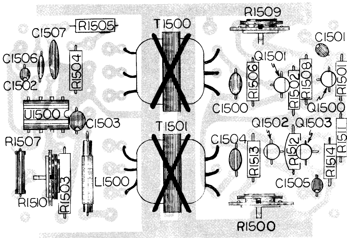
Figure 5-23. BFO and Line Amplifier, P/N 689-1500 (A15)
