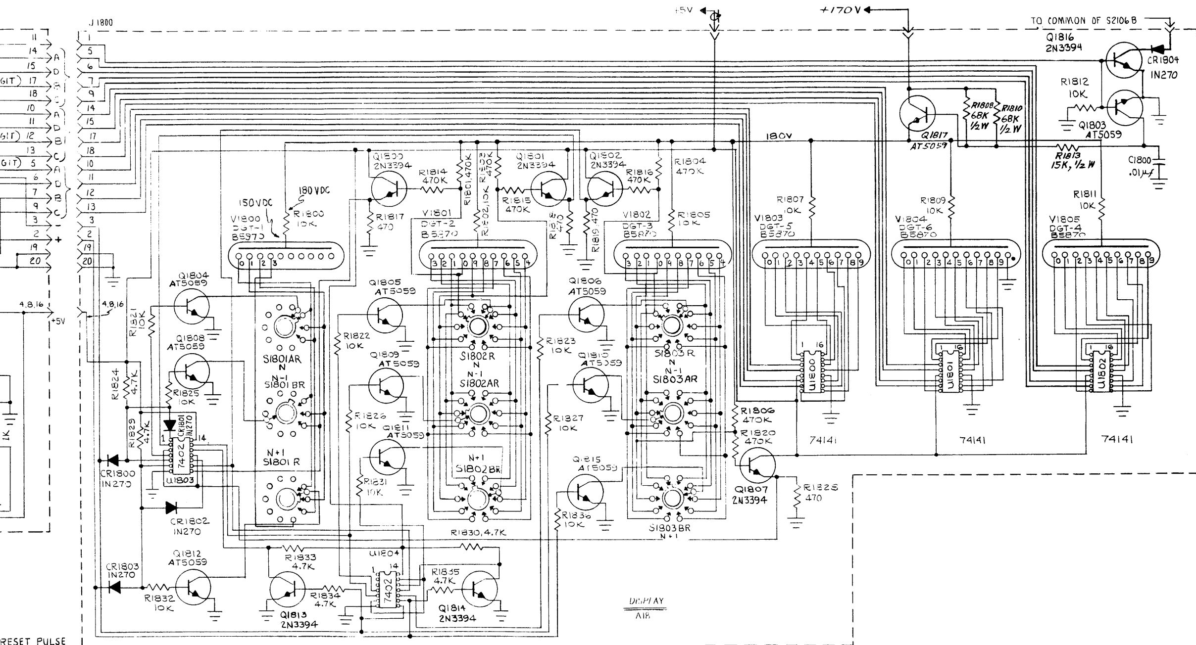
Figure 5–35. Counter Schematic
