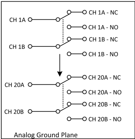
Typical Channel
