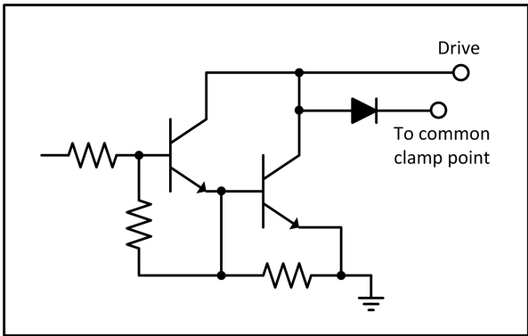
Typical Darlington Channel (1 of 32)
