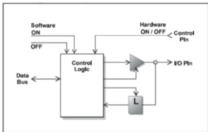
Typical Drive Channel
