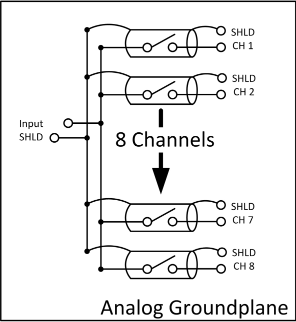
Typical 1x8 (1 of 12)
