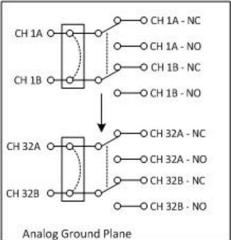
Typical Diagram for one DPDT Relay
