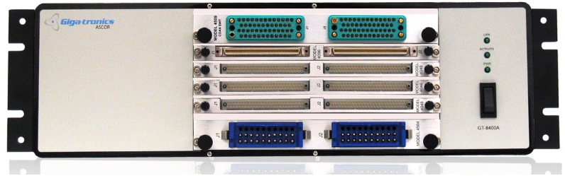
4000 Series Switch Modules with GT-8400A Chassis
