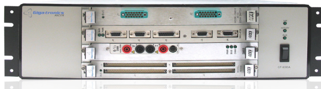
Low Cost GT-8300A 3U chassis with LAN and IEEE-488 Control
