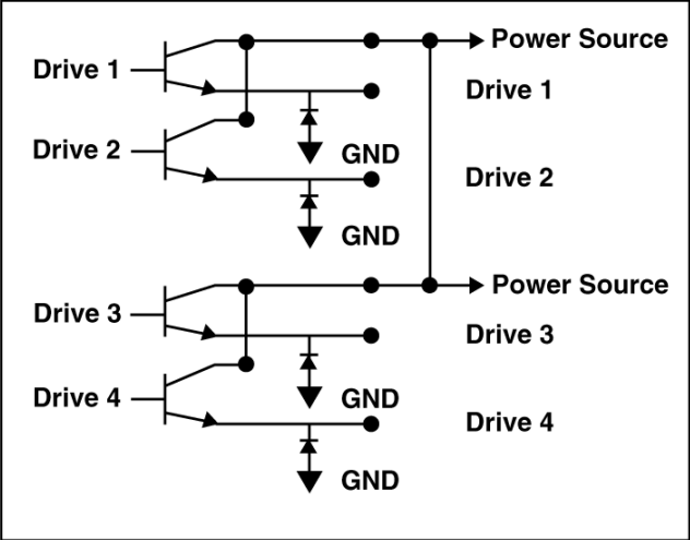
4 of 16, Typical Driver Channels
