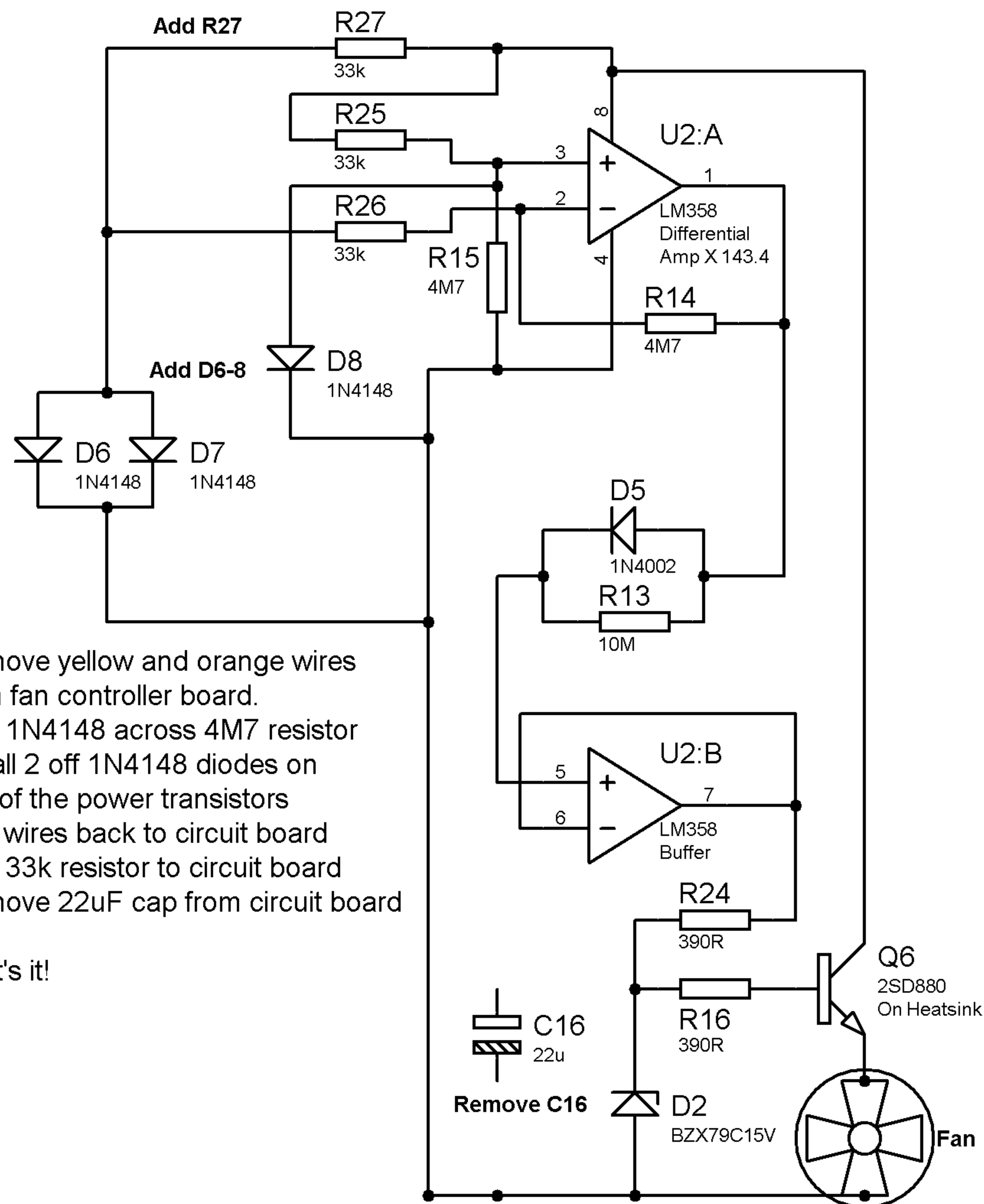
After Modification
